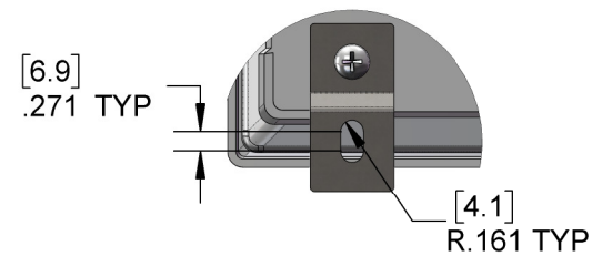
DETAIL A SCALE 1 : 3
